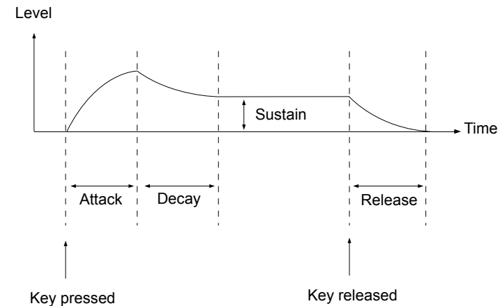
Figure 4.8: The amplitude envelope.
