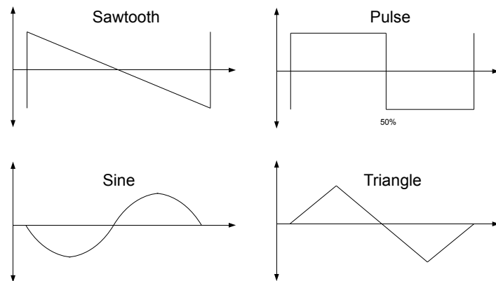
Figure 4.2: Basic oscillator waveforms.
