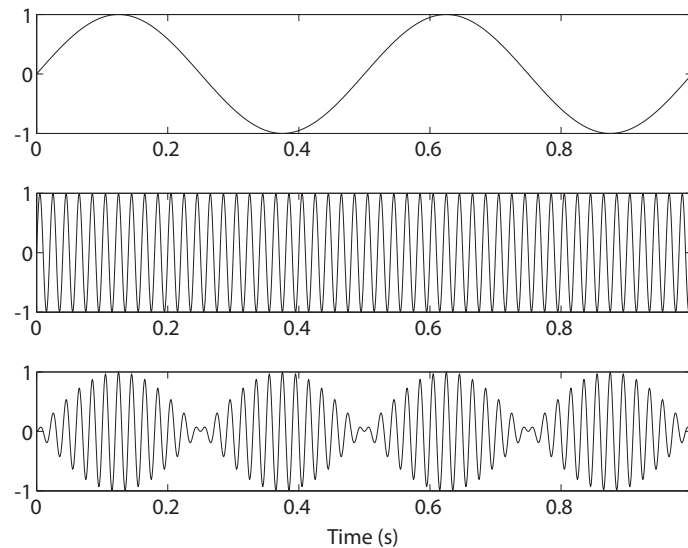
Figure 4.5: Ring modulation of two sine waves.
