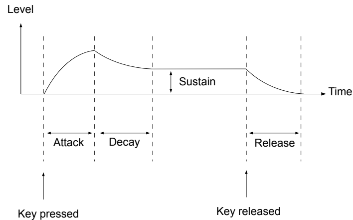
Figure 4.7: The filter envelope.
