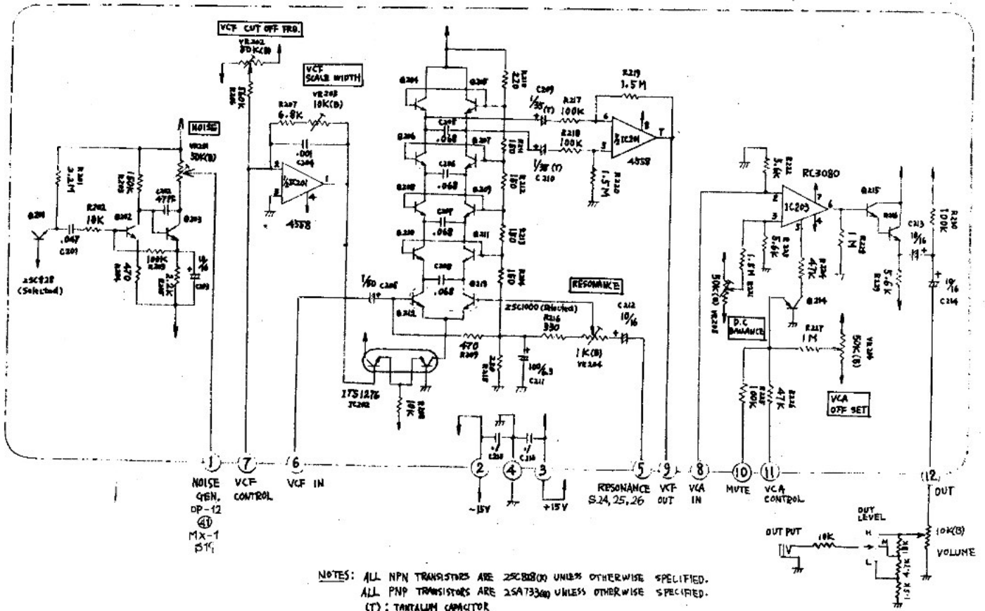
6-2. VCF-2 Circuit Diagram
