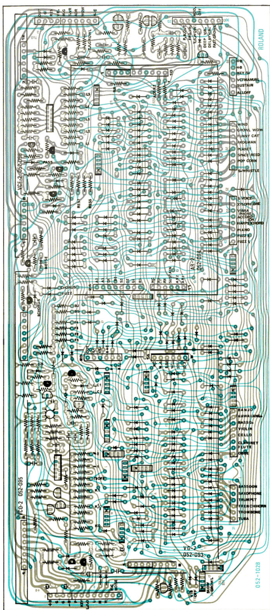
9-5. Both Side Circuit Patterns of MX-1 Board
