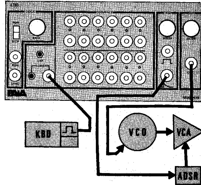
Figure 4 - GENERATING ARPEGGIO AS EACH KEYBOARD KEY IS RELEASED
