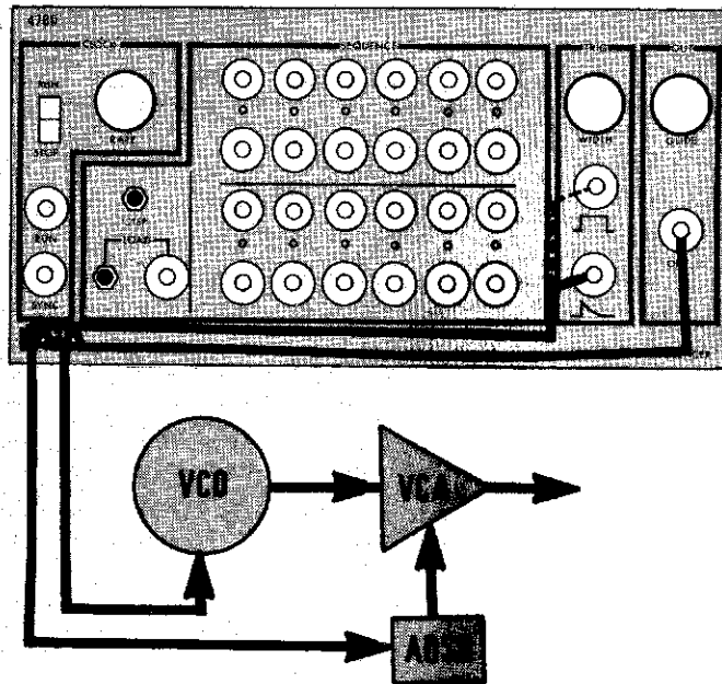
Figure 1 - COMMON SEQUENCER PATCH
