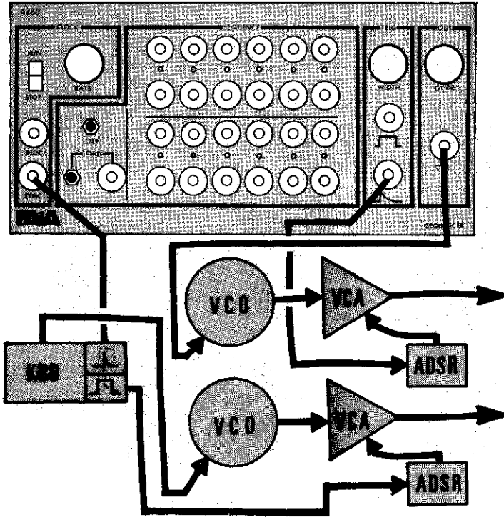
Figure 3 - SYNCHRONIZING SEQUENCER TO KEYBOARD
