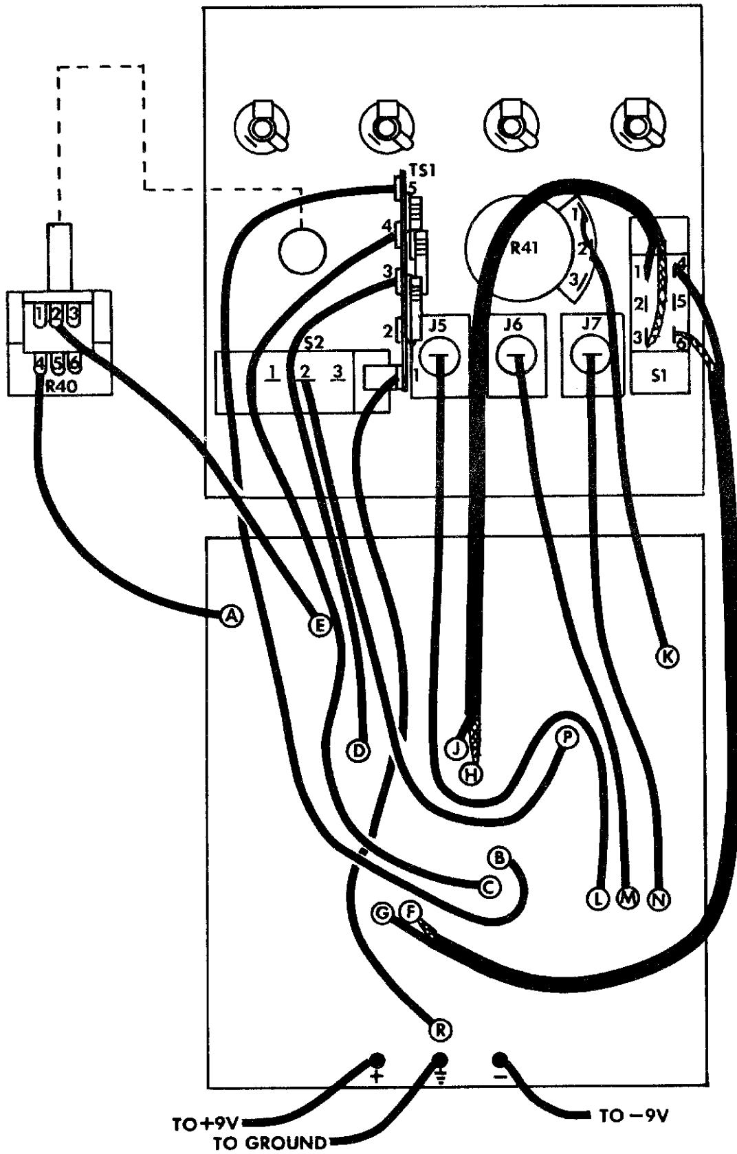
Figure 9 - Circuit board to front panel wiring detail. Previous wiring has been omitted for clarity.
