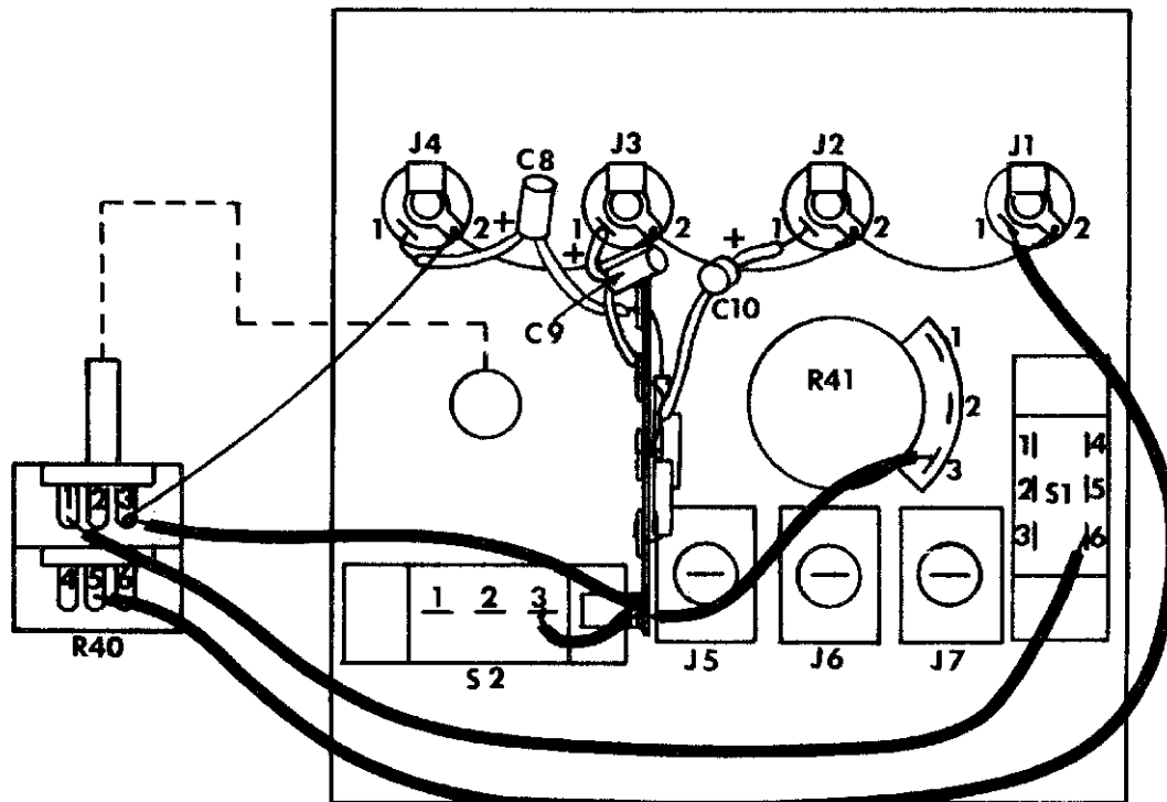
Figure 4 - Front panel layout and wiring.
