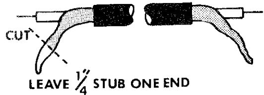
Figure 2 - Co-ax detail.
