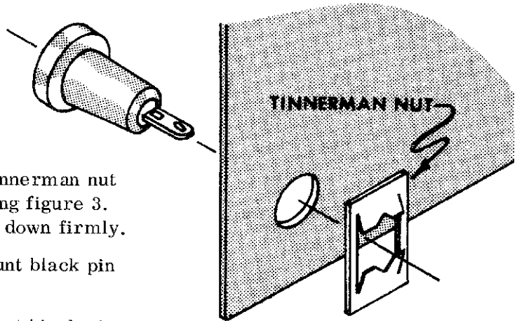
Figure 3 - Tinnerman nut mounting detail.
