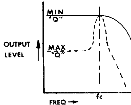
Figure 14 - Effect of varying Q on Low-Pass output
