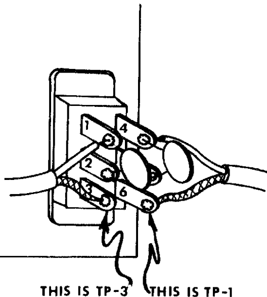
Figure 11 - Test points.
