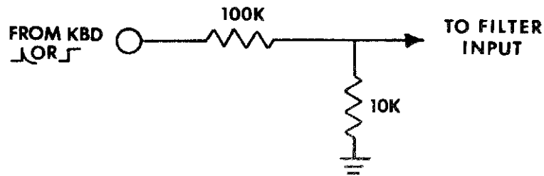
Figure 15 - An attenuator is required to apply keyboard triggers to 4730 audio inp
