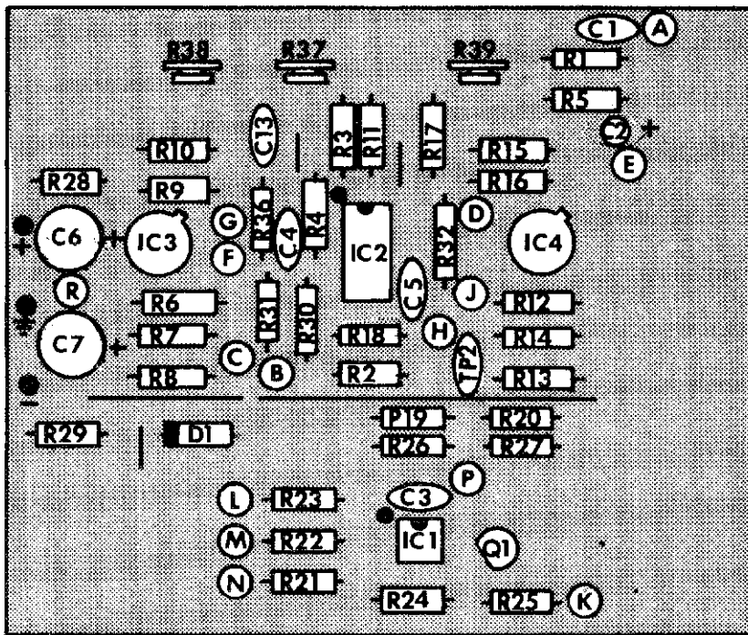
Figure 1 - Circuit board parts placement.
