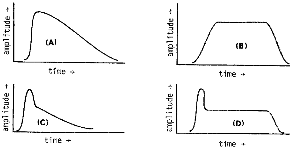
FIGURE 1. Amplitude envelopes for (A) Percussion (B) reeds (C) attack-decay-release (D) attack-decay-sustain-release
