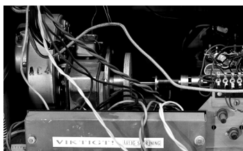
A close-up view of the main 60Hz motor. The vibrato scanner is mounted on the left side.
