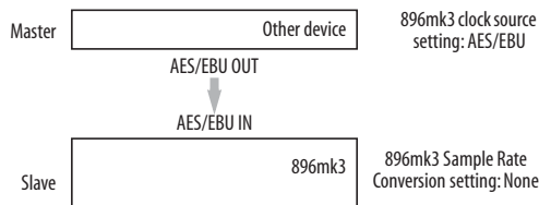
Figure 3-13: Slaving the 896mk3 to an AES/EBU device. For the 896mk3's clock source, choose 'AES/EBU'.
