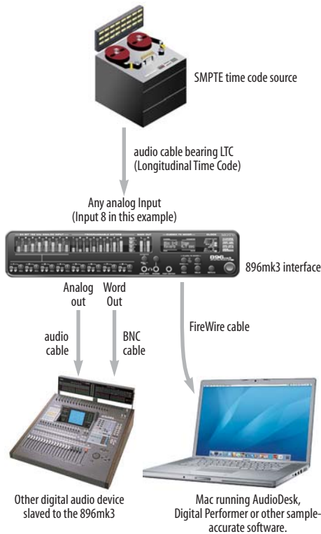
Figure 3-8: Connections for synchronizing the 896mk3 directly to SMPTE time code.
