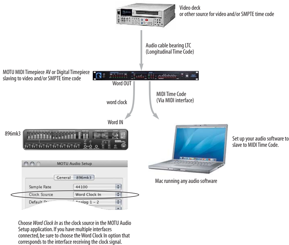
Figure 3-9: If your host audio software does not support sample-accurate sync and the 896mk3's built-in SMPTE sync features, use a universal synchronizer such as the MOTU MIDI Timepiece AV or Digital Timepiece.
