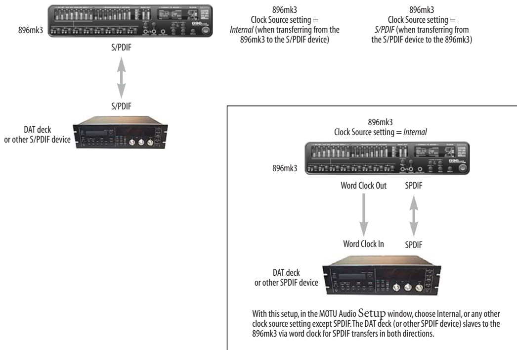
Figure 3-10: Two setups for synchronizing an S/PDIF device with the 896mk3. In the top diagram, sync is achieved via the S/PDIF connection itself. In this case, you have to choose S/PDIF as the 896mk3's clock source when recording from the S/PDIF device. If you don't want to have to worry about switching the Clock Source setting depending on the direction of the S/PDIF transfer, you can slave the S/PDIF device to word clock from the 896mk3 or vice versa (not shown). The Word Clock connection maintains sync, regardless of the direction of the transfer.
