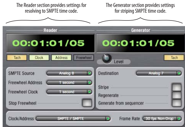
Figure 12-1: SMPTE Setup gives you access to your 896mk3's on-board SMPTE time code synchronization features.
