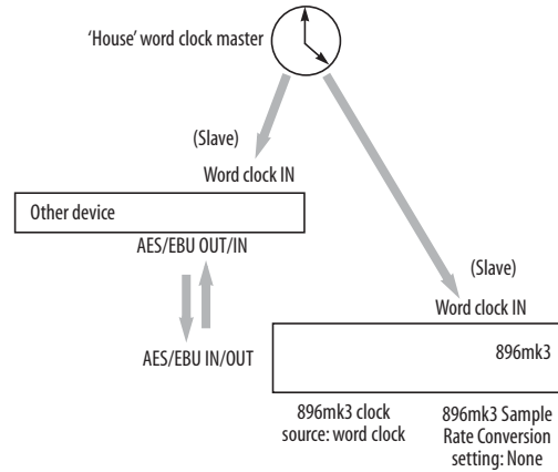
Figure 3-15: In this scenario, the 896mk3 and other AES/EBU device are both resolved to one another via a third master word clock source.
