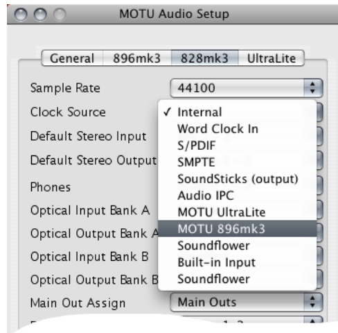
Figure 3-21: To resolve a MOTU FireWire interface to another Core Audio device, choose the other device from the Clock Source menu in the MOTU FireWire Audio Console. In this example, the 828mk3 will slave to the 896mk3.
