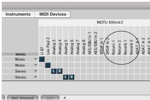
Figure 7-2: The stereo return and reverb return busses from the 896mk3 in Digital Performer's Bundles window.
