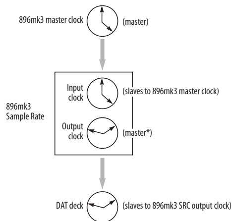
Figure 3-12: Clock relationships when sending audio from the 896mk3 to a DAT deck using sample rate conversion. The DAT deck needs to be slaving to its AES/EBU input. *Note: the 896mk3 AES/EBU output can actually be clocked from a number of different sources. In this example, it is resolved to the 896mk3 system clock. For details about other possible clock sources, see “Clocking scenarios for AES/EBU output” on page 27.
