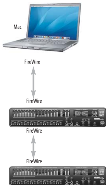
Figure 3-19: Connecting multiple 896mk3's (or other MOTU FireWire audio interfaces) to a computer.
