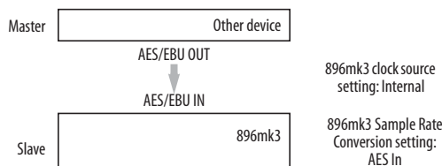
Figure 3-14: Rate-converting AES/EBU input.
