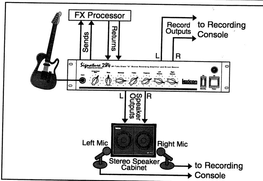
Recording with direct outputs and microphones
