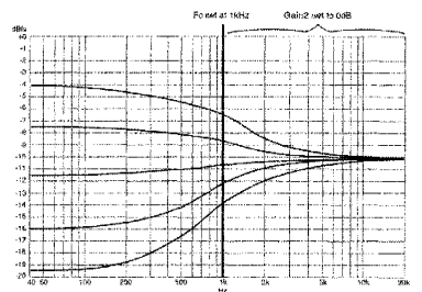
Setting Gain 2 to 0dB creates a simple bass control
