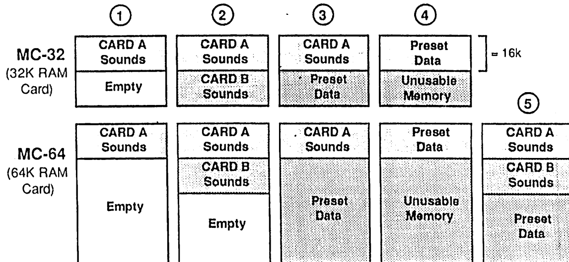
Possible RAM Card Configurations
